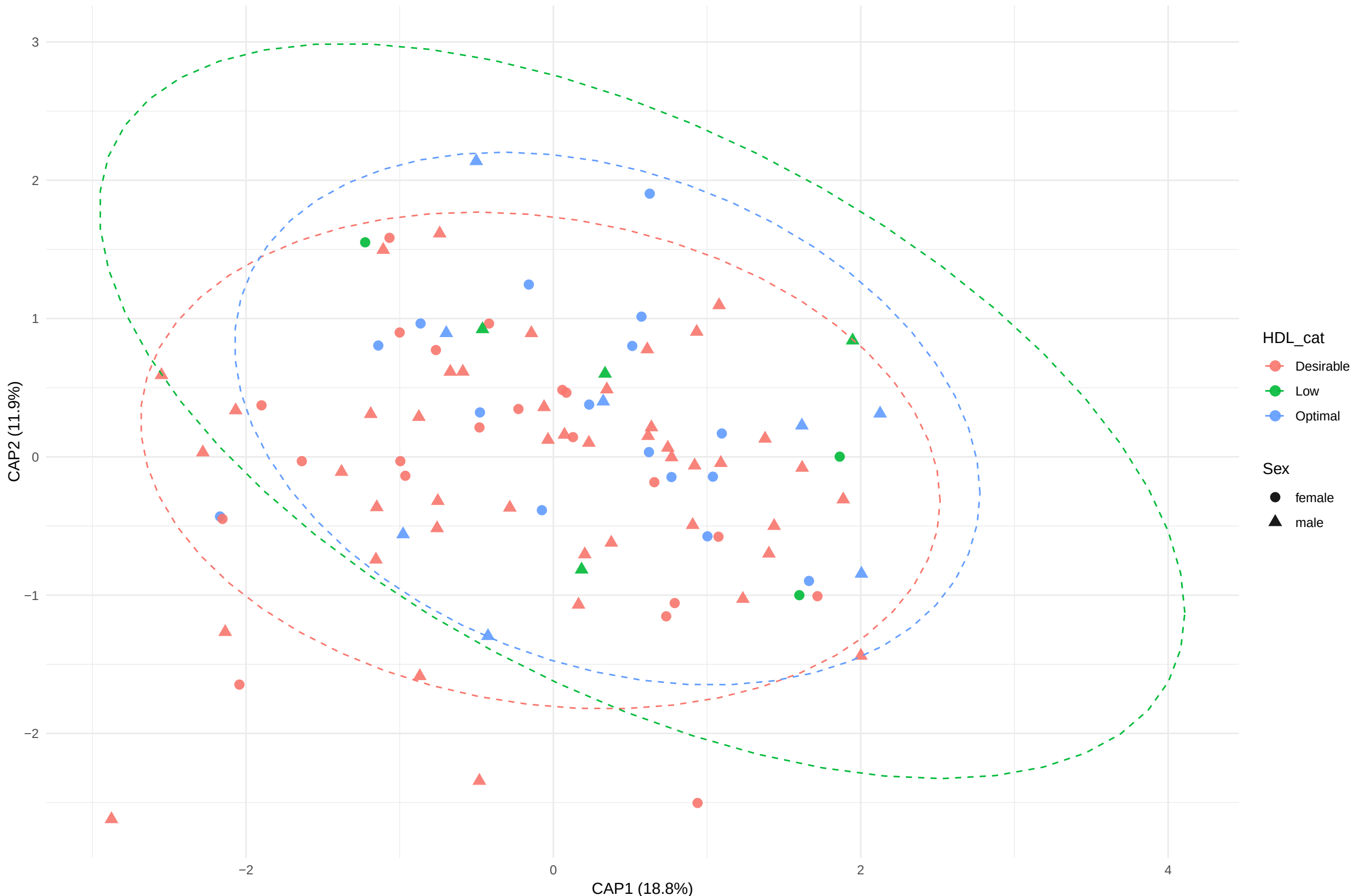
CAP Ordination by Multiple Variables adonis R 2 = 0.17, p = 0.365
